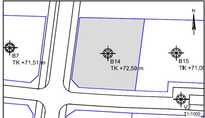
Figur 1 – Situationsplan 1:1000, Parcel nr. 14
