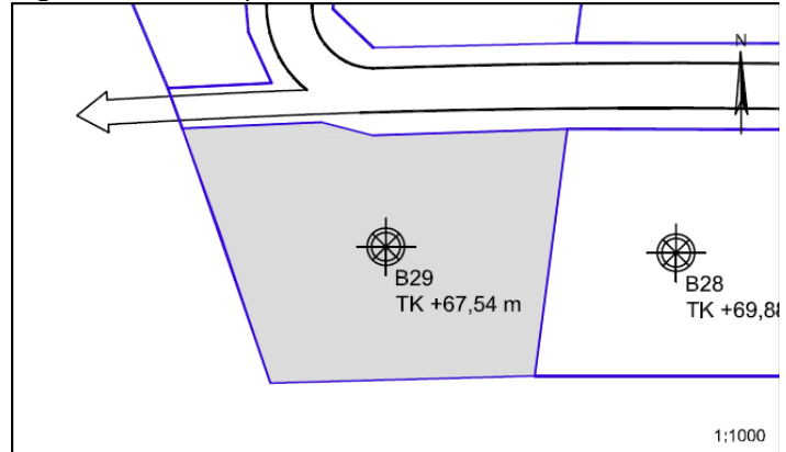
Figur 1 – Situationsplan 1:1000, Parcel nr. 29
